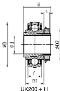
UK200 + H
