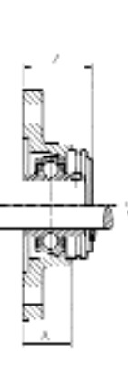
UCFL200CO(CC)
