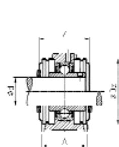
UCPG200CO(CC)
