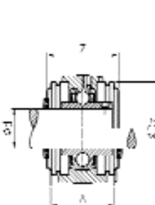
UCP200CO(CC)
