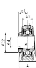
UKPE200H
