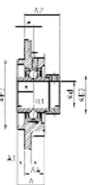
EXFC200
