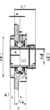
EXFC200
