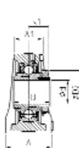
UKP200H UKP300H
