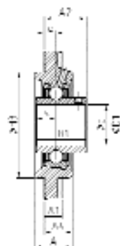
UCFS300
